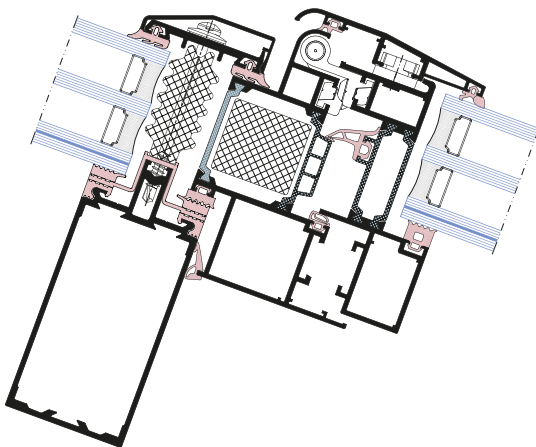
Roof windows AF 50R in the facade AF 50
