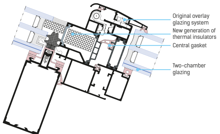
Roof windows AF 50R in the facade AF 50S
