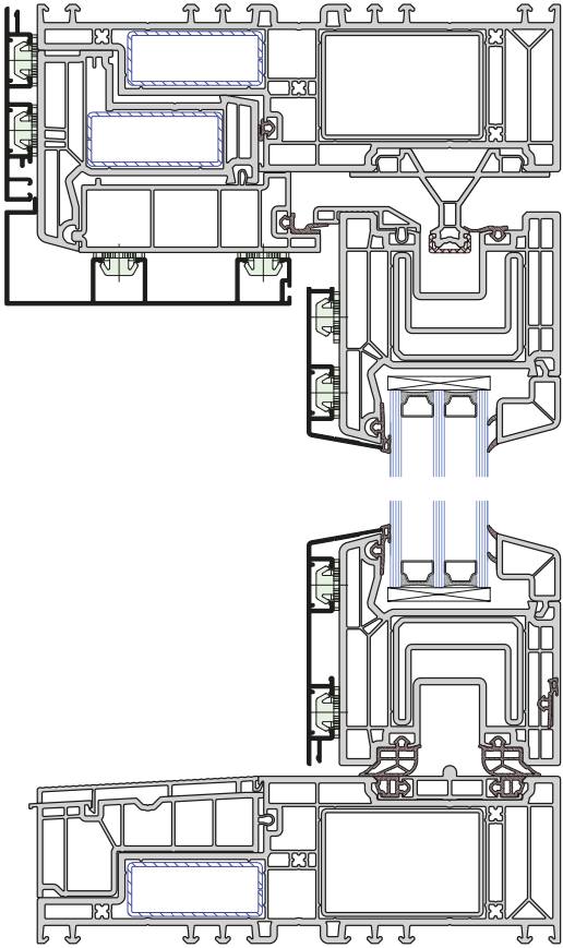
Vertical cross-section through the fixed sash
