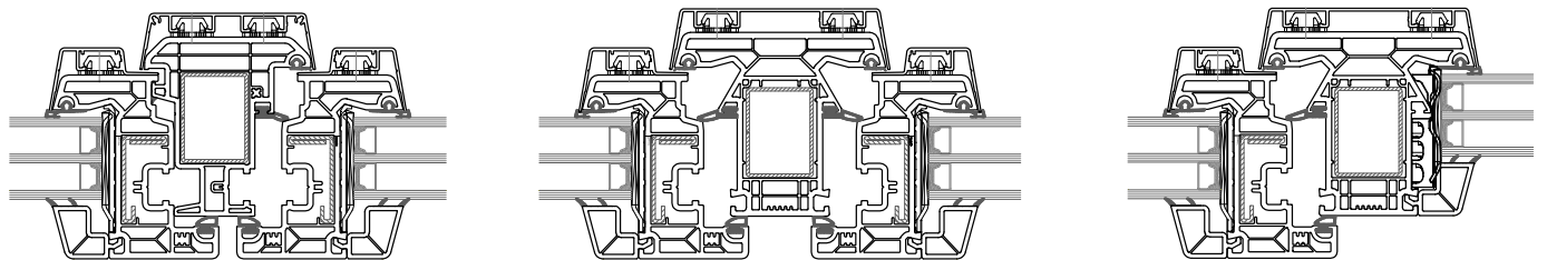
Flying mullion, fixed mullion, transom bars
