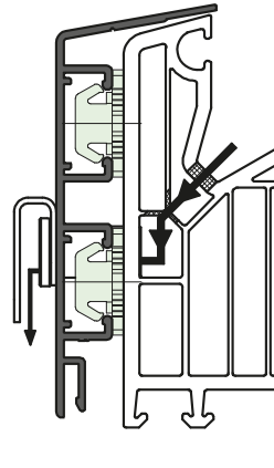
Fig. 3 - Water drainage - front + aluminium end plug
