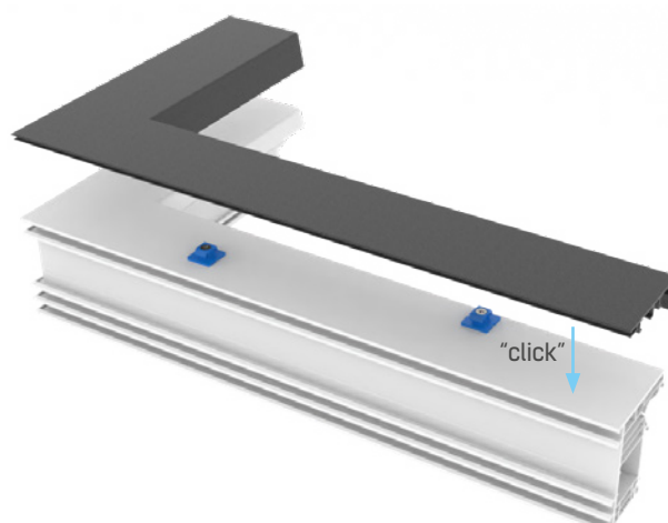
Assembly of aluminium frames with clips
