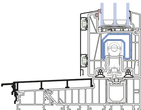
Vertical cross-section through the active sash
