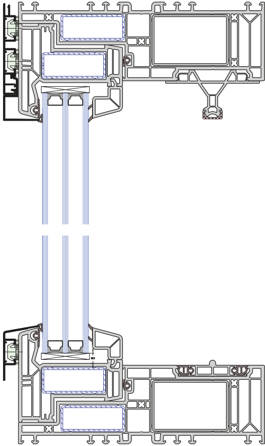
Vertical cross-section through the active sash
