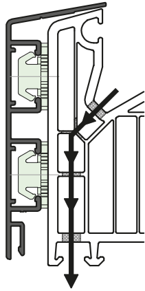
Fig. 2 - Water drainage - bottom
