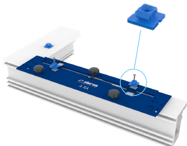
GEMINI system assembly templates
