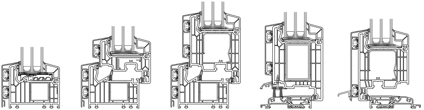
Fixed glazing, single-leaf windows and doors
