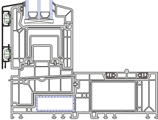
Vertical cross-section through the fixed sash
