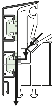
Fig. 1 - Water drainage - front
