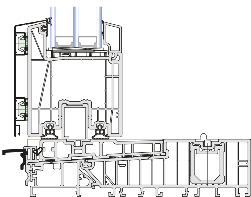
Vertical cross-section through the fixed sash
