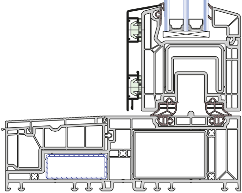
Vertical cross-section through the active sash
