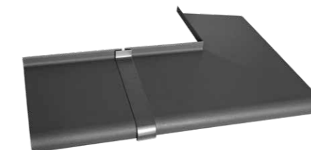
Straight connector 180° (LAS/XXX)
