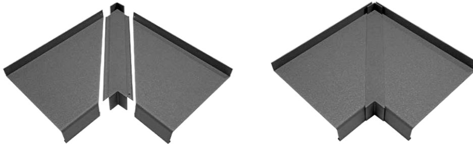
Internal corner connector 90° (LAK40/XXX/W/90S)
